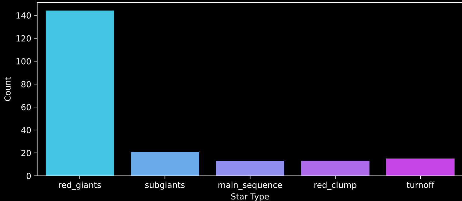
APOGEE DR17 Field: [225-04] Count plot of Star Type
