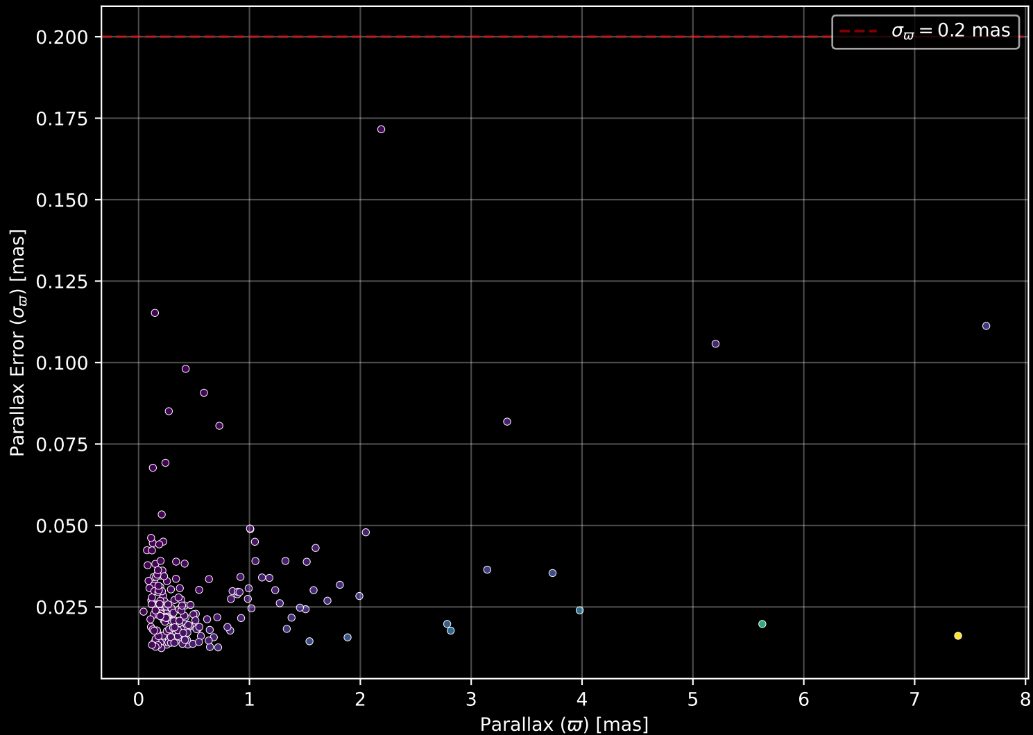
APOGEE DR17 Field: [225-04] Parallax Quality (n= 206)
