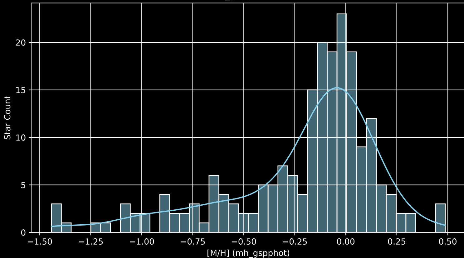
APOGEE DR17 Field: [225-04 [M/H] (mh_gspphot) (n= 202)
