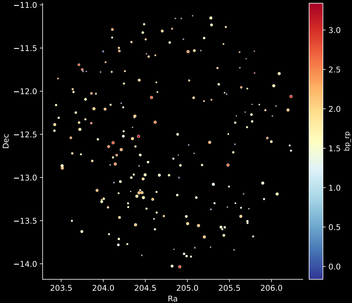
APOGEE DR17 Field: [225-04] Stars: 206
