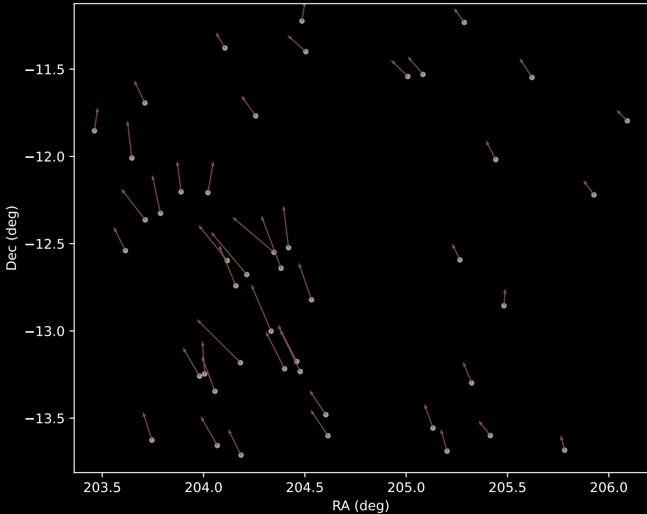
APOGEE DR17 Cluster 10 Proper Motion Vectors (n=46)
