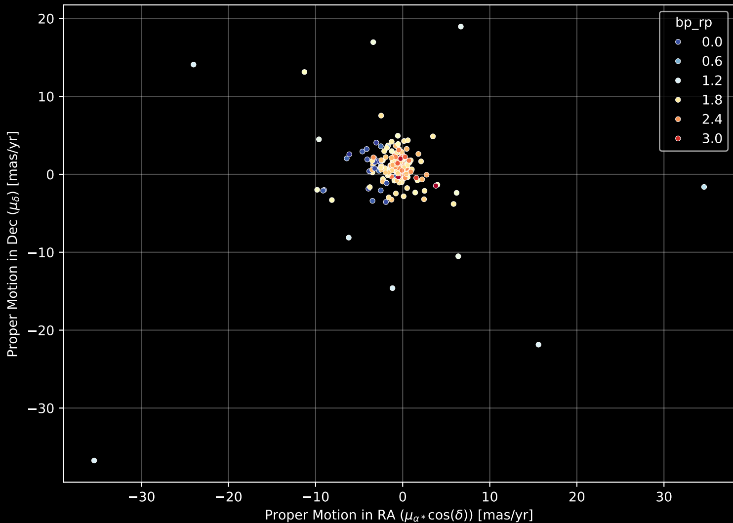
APOGEE DR17 Field: [225-04] Proper Motion Diagram (n= 206)
