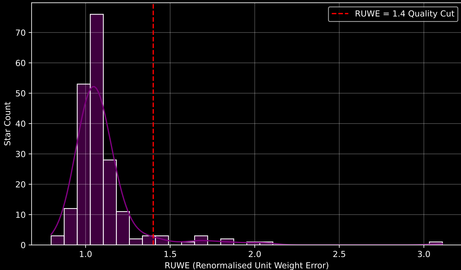
GAPOGEE DR17 Field [225-04] RUWE Distribution (n= 200)
